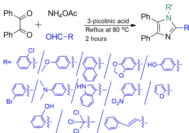
Scheme 1 Reaction for three substituted imidazole synthesis.
