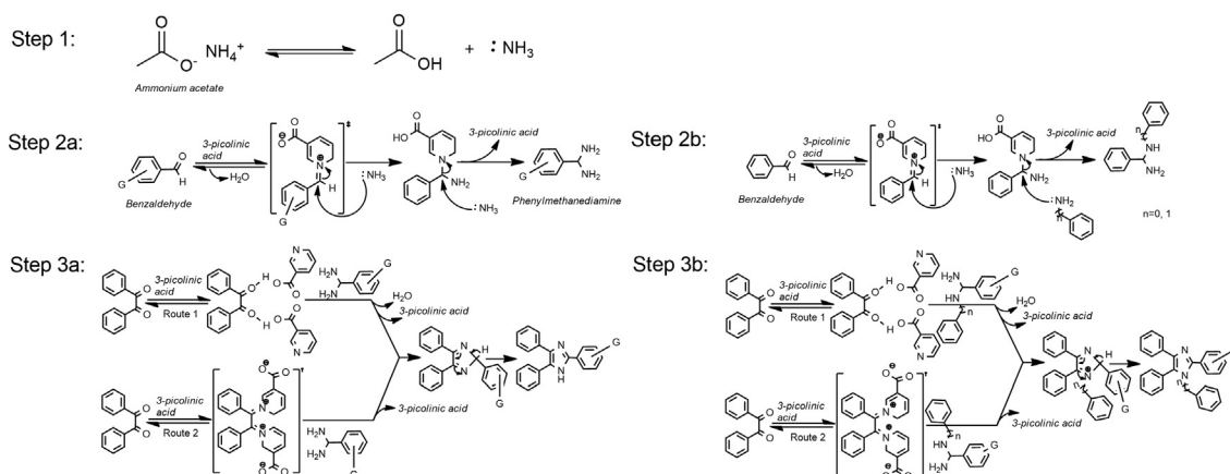
Fig. 1 The stepwise mechanistic pathway for the multi-substituted imidazole synthesis via one-pot, three, and four components condensation reaction mediated by 3-picolinic acid.
