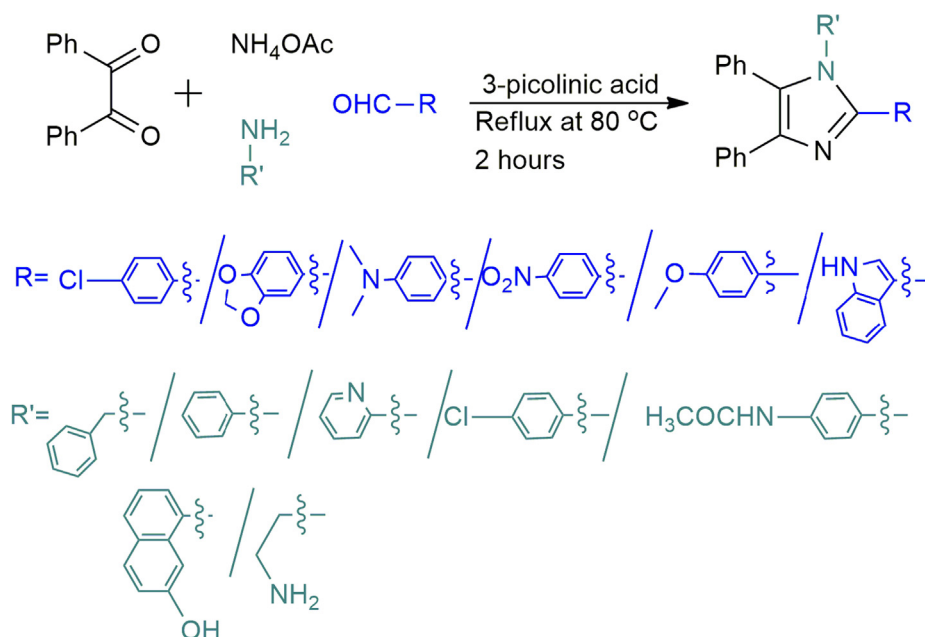
Scheme 2 Reaction for four substituted imidazole synthesis.
